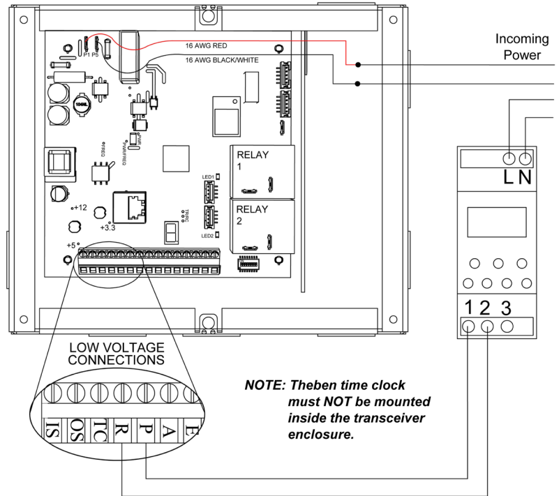
Figure 7 Transceiver With 7-Segment Display
